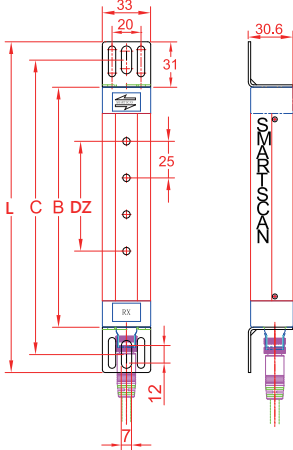
NA Dimensions
