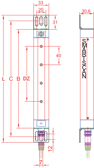
NA Dimensions
