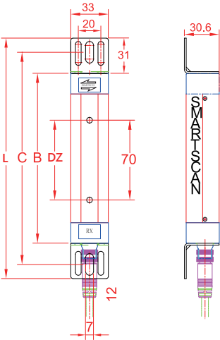
NA Dimensions
